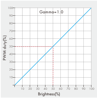
Dimming curve
