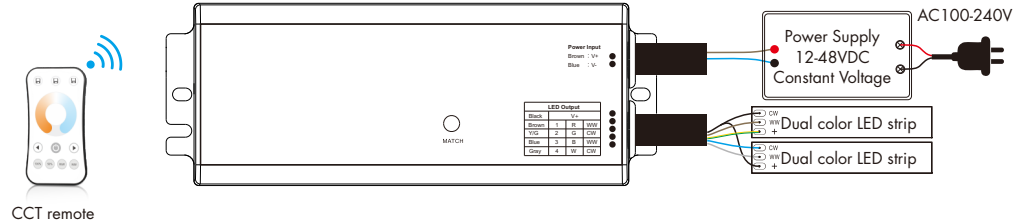
CCT remote
