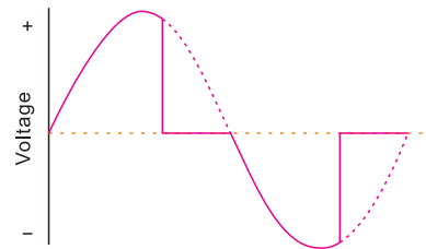
Reverse-phase control dimmer
