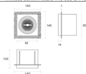
Trimless 50mm Fixture 148-060 &amp; 148-061
